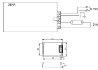
Scheda tecnica Philips HID-PV C 70 /S CDM 220-240V 50/60Hz
